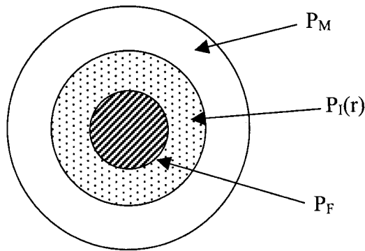
Figure 1 Transverse schematic of the three-layer interphase model proposed by Theocaris.
