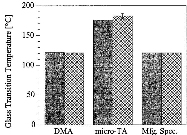
Figure 2 Measured glass transition temperatures ( T_g ) for commercial aerospace resin system on glass (solid gray) and carbon (cross-hatched).
